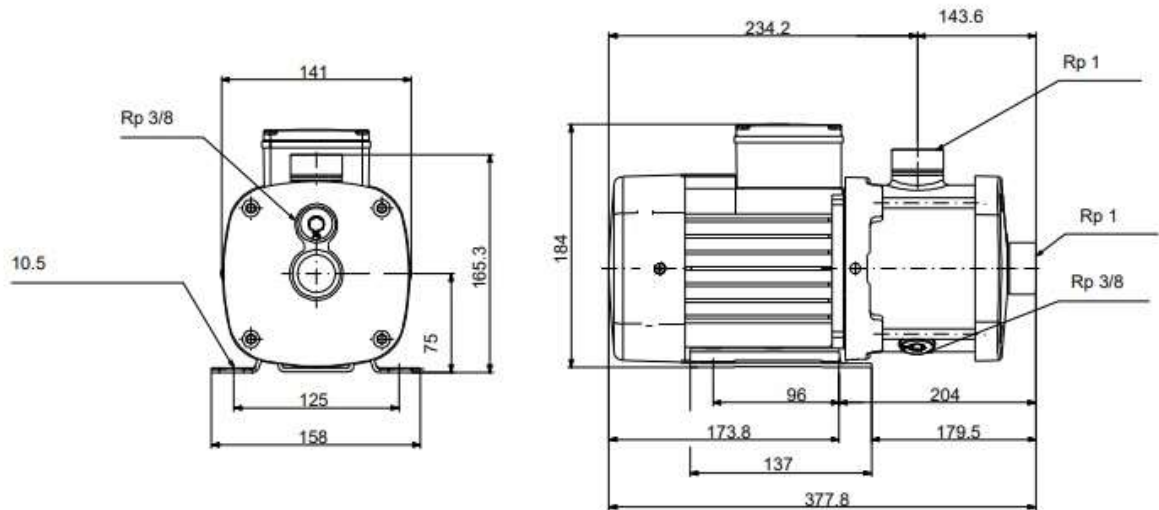
DIMENSIONAL DRAWING OF WATER PUMP (All dimensions are in mm)
